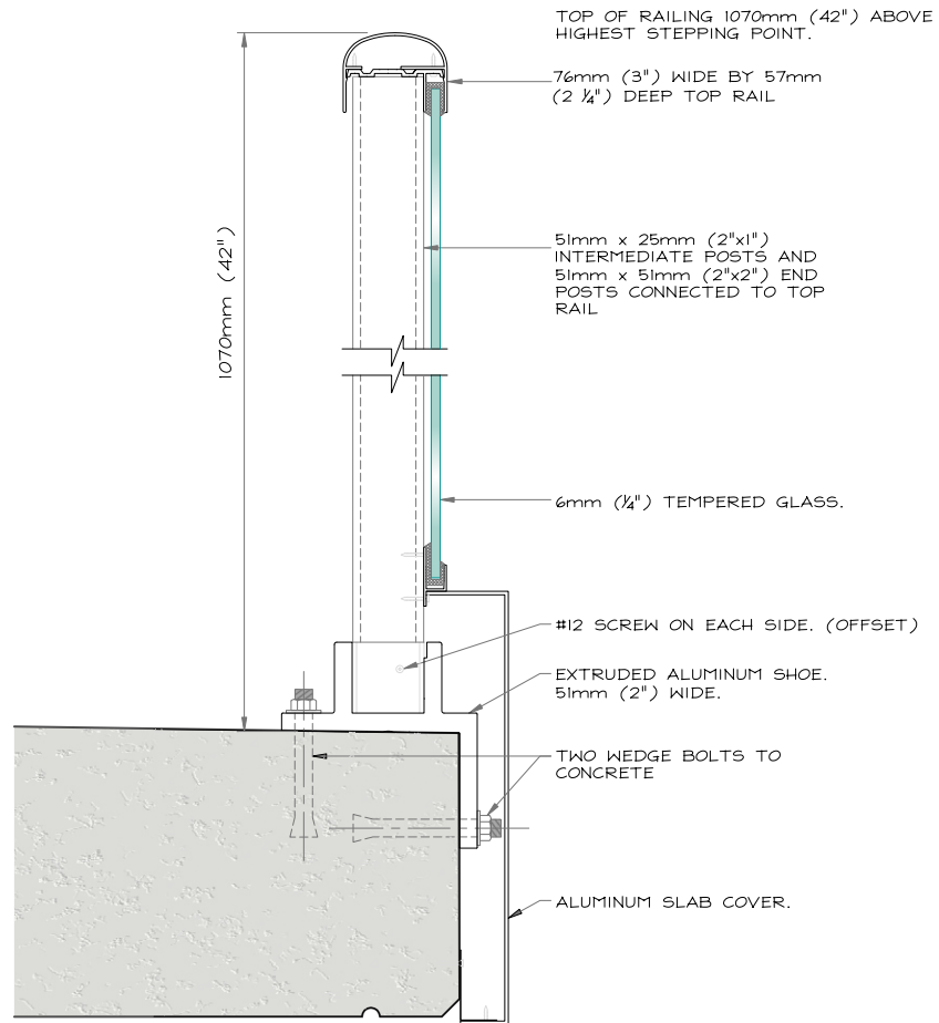
Balcony Railings on Concrete Slab with Metal Slab Cover
