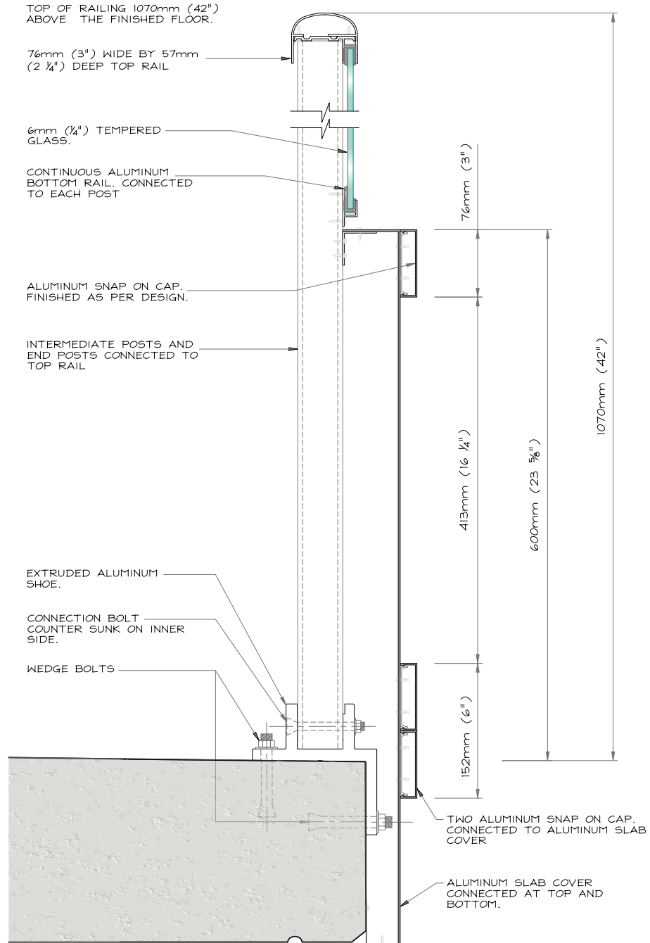
Balcony Railings on Concrete Slab with Extended Metal Panel & Slab Cover
