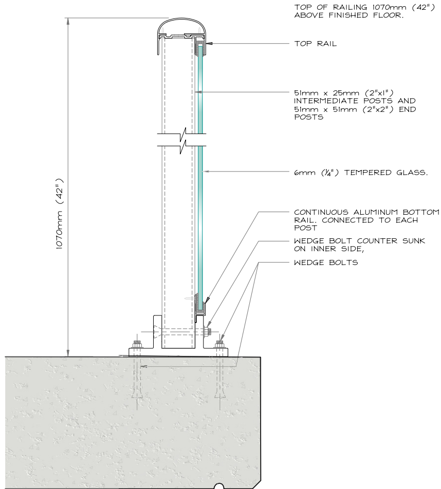
Recessed Balcony Railings on Concrete Slab
