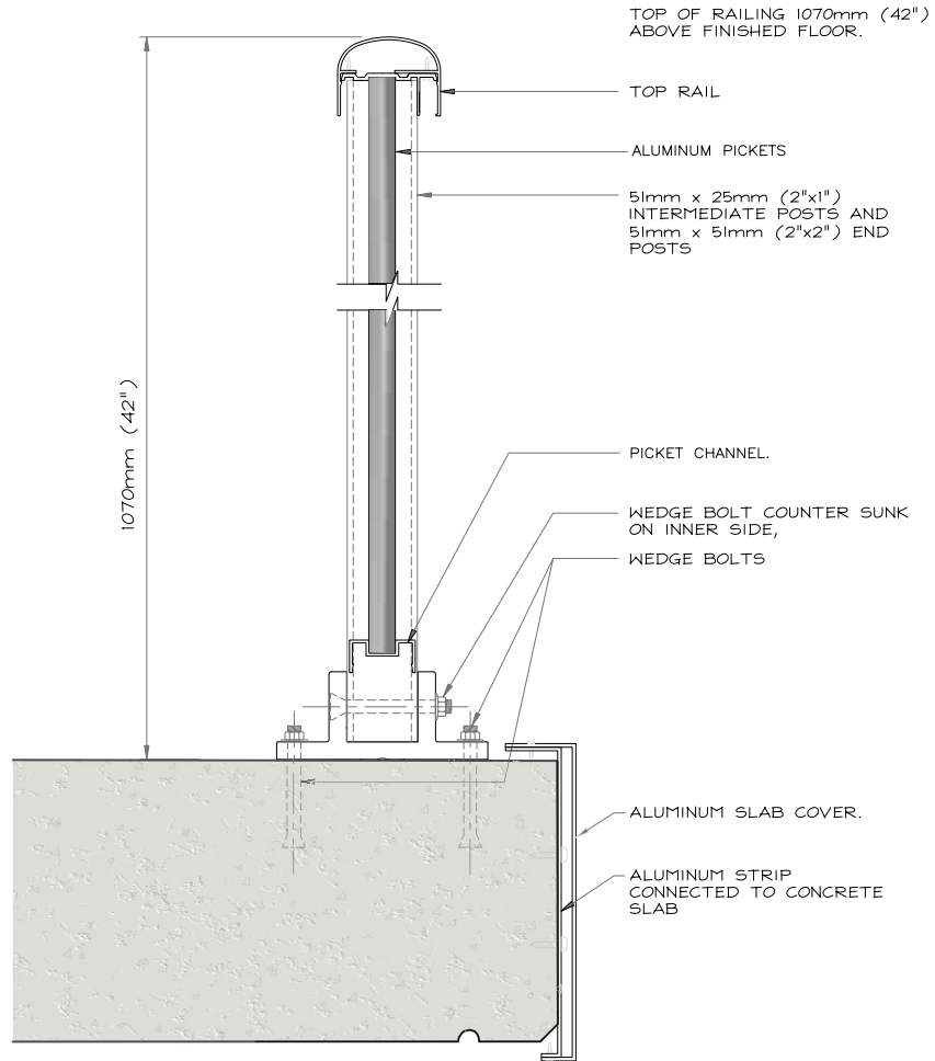
Aluminum Picket Balcony Railings with Metal Slab Cover
